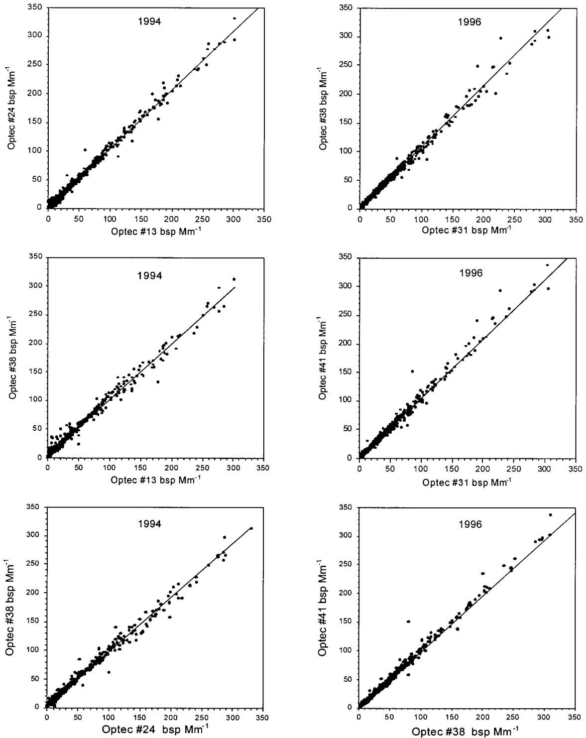
Figure 7. 1994 and 1996 Optec NGN nephelometer intercomparisons of hourly average aerosol scattering (regression statistics are listed in Table 2).
