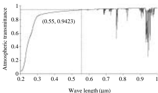
Fig. 3. Calculated atmospheric transmittance at the wavelength of 550nm using MOTRAN 4.
