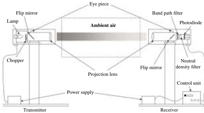
Fig. 1. Function diagram of a transmissometer.
