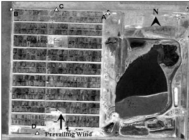
Figure 1. Overhead photograph of the cooperating feedyard. Instruments were deployed so that we could measure PM 10 and TSP mass concentration and atmospheric extinction simultaneously measured along the downwind boundary of the feedyard. Transmitter is at A, receiver (photometer) is at B, upwind TEOM is at D, and downwind TEOMs are at C.
