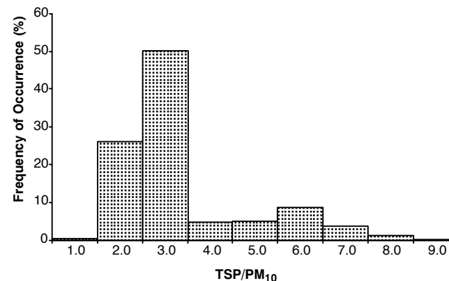
Figure 11. Frequency distribution of TSP/ \text{PM}_{10} ratio for all measured data.
