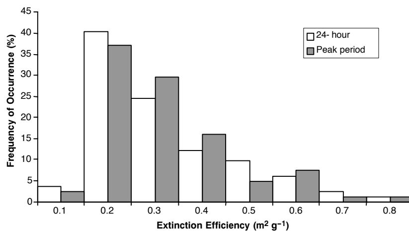
Figure 6. Frequency distribution of extinction efficiency ( \text{m}^2 \text{g}^{-1} ) for downwind TSP during 24-hour intervals and dust-peak periods from September 2005 to July 2006.
